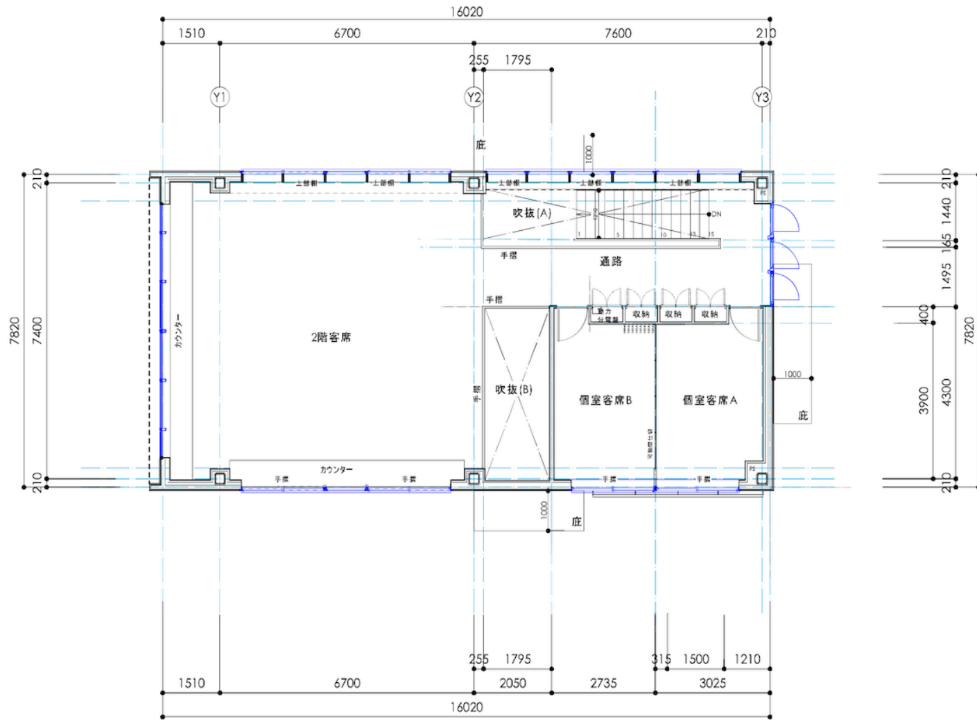
2F PLAN
