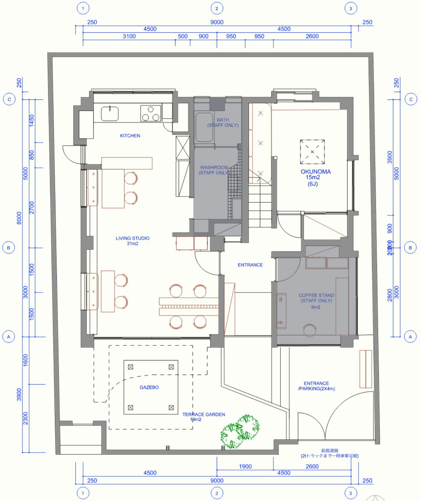
1F PLAN
