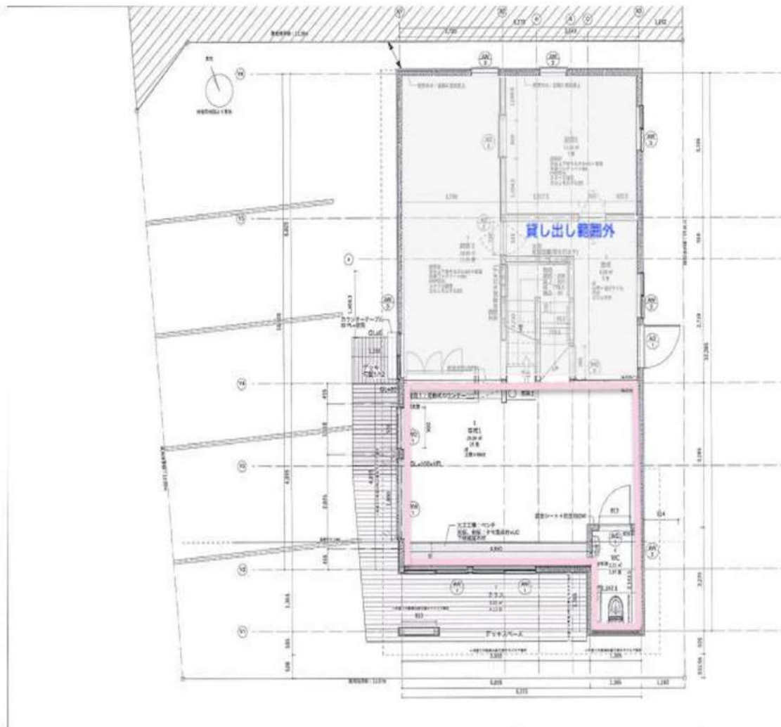
1F PLAN S-1/60
